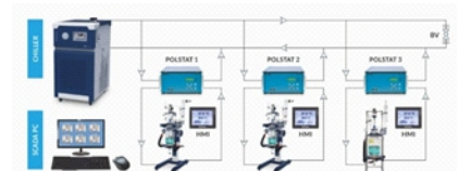
Distributed Temperature Control Unit
